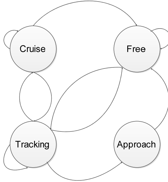
Figure 8: System Finite State Machine Graph
